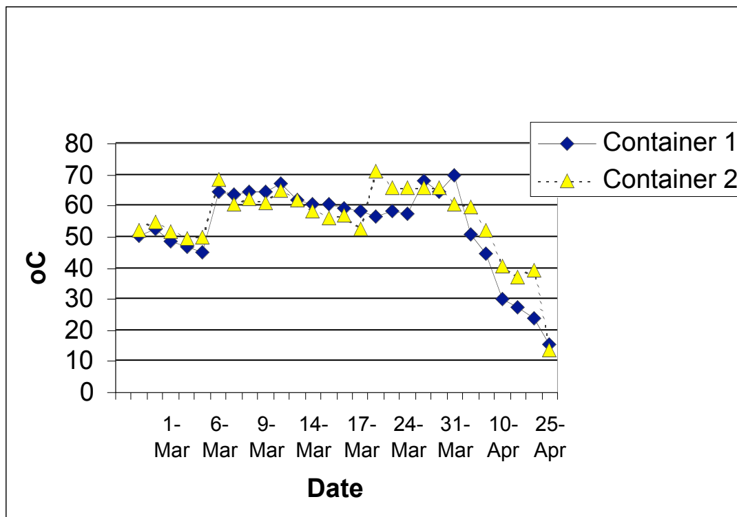
Figure 1. Temperature development in the two composts
