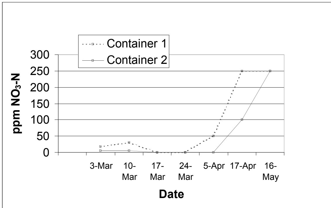
Figure 3. Development of NO 3 - N in the two composts
